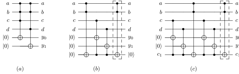
Fig. 5. Circuits for function y_0 = abc, y_1 = abd . (a) Initial circuit. (b) An equivalent circuit constructed by reusing ab as a shared cofactor. (c) When no unused zero-initialized output exists. Gates in dashed box are used to un-compute the cofactor ab .
