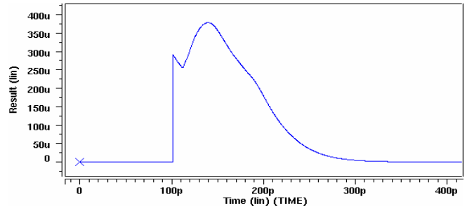
Figure 5. Total current flowing to ground while turning on the circuit.
